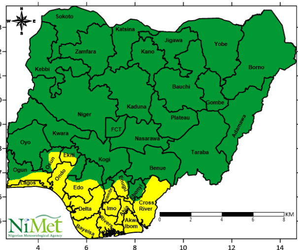
Fig 1.0: Spatial display of rainfall and probability valid from 0000UTC of 6 TH NOVEMBER to 2359UTC of 6 TH NOVEMBER, 2024.
